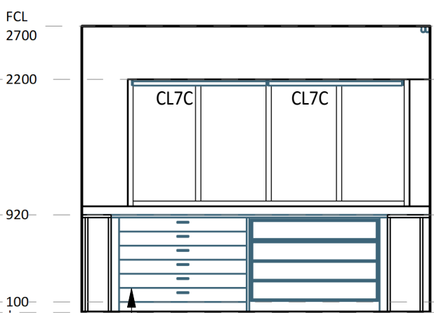
7 ELEVATION DETAIL 1 : 50
