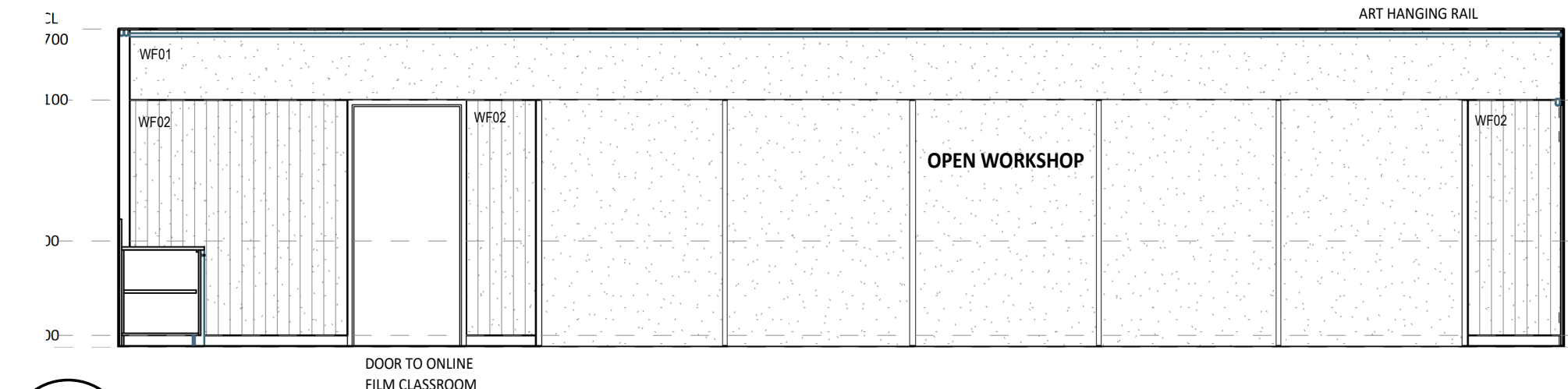
5 ELEVATION DETAIL 1 : 50
