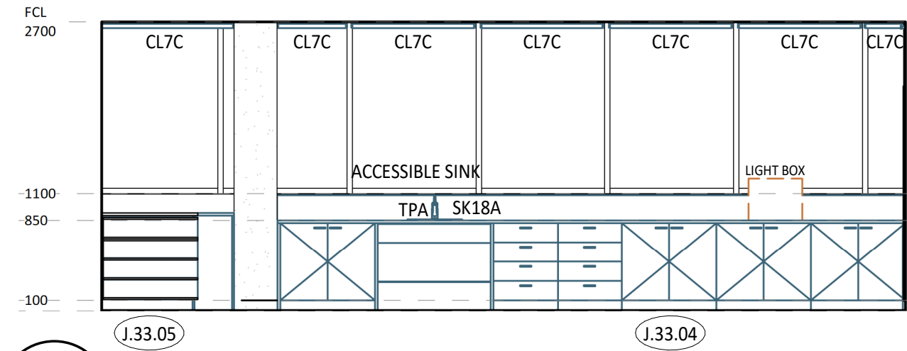
4 ELEVATION DETAIL 1 : 50
