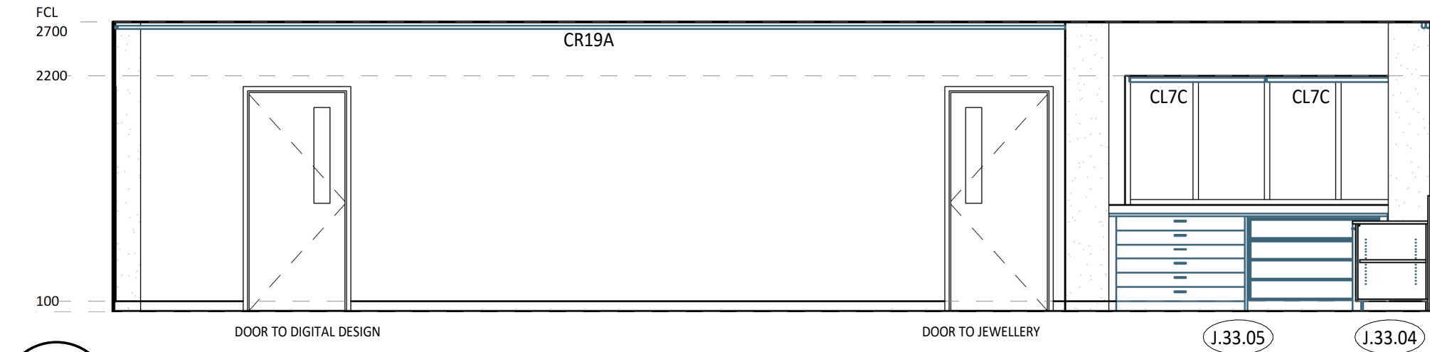
3 ELEVATION DETAIL 1 : 50
