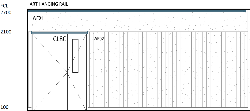
6 ELEVATION DETAIL 1 : 50
